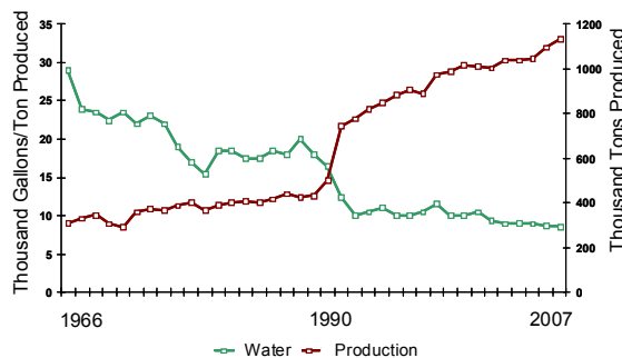
Fig. 1. Water use in paper production (MWV Mahrt mill, 1966 – 2007)
